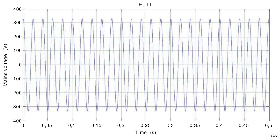
a) Mains signal with modulation d = 0,407\% at 13,5\text{ Hz} ( P_{st}^V = 1 )
