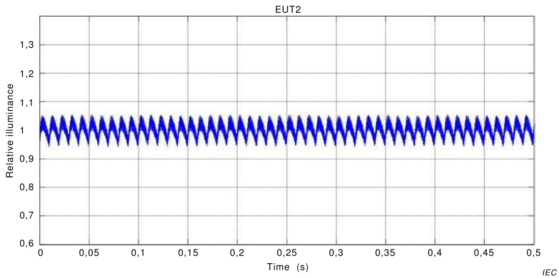
Figure C.4 – EUT2: relative illuminance: mains voltage modulation d = 0,407\% at 13,5\text{ Hz} ( P_{st}^V = 1 )
