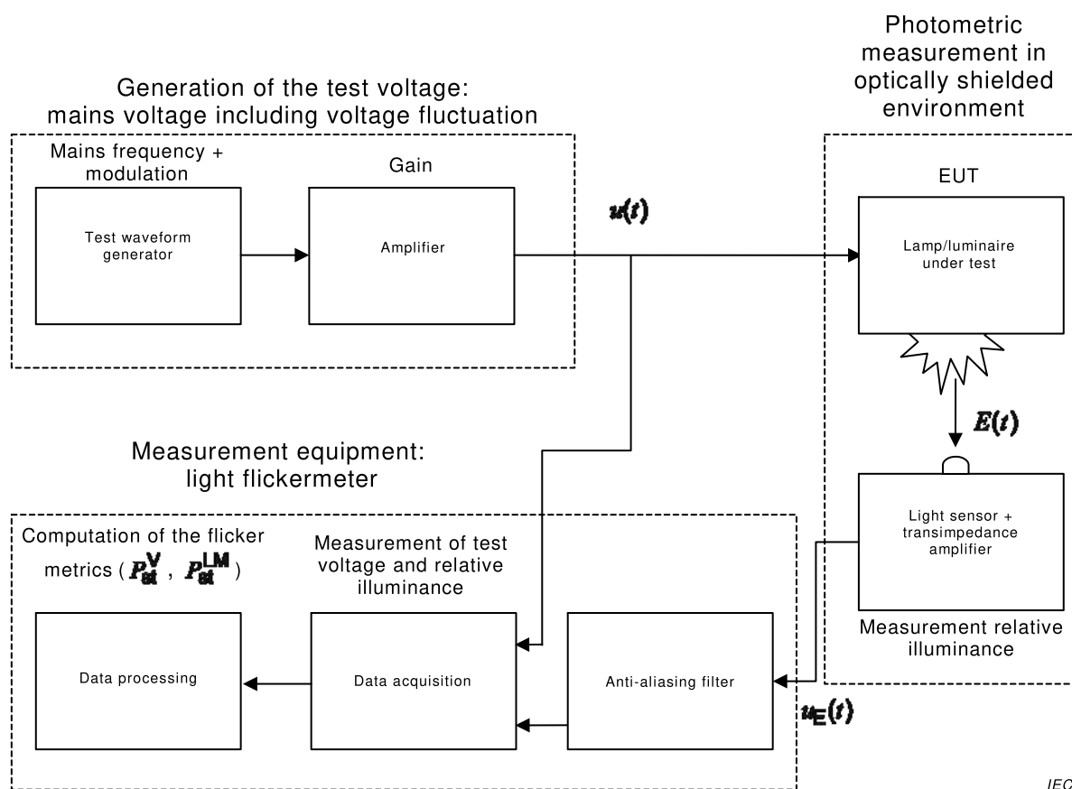
Figure 3 – Block diagram voltage-fluctuation immunity test
