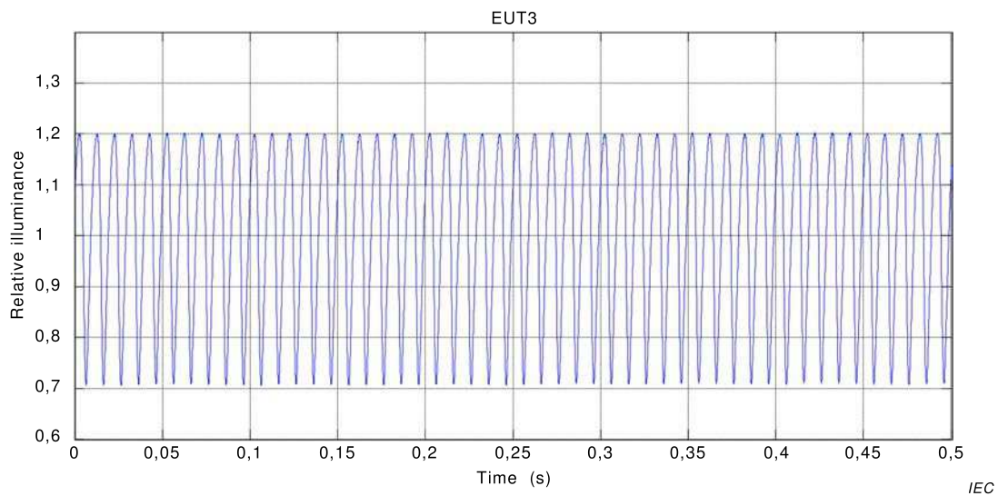
Figure C.5 – EUT3: relative illuminance: mains voltage modulation d = 0,407\% at 13,5\text{ Hz} ( P_{st}^V = 1 )
